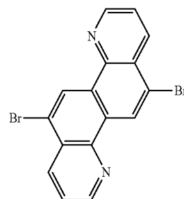
Intermediate compound 1
